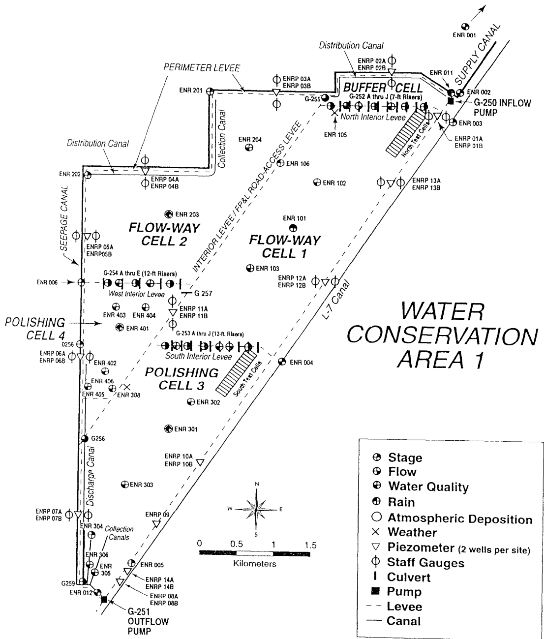
Figure 1-2. Everglades Nutrient Removal Project Site Plan and Monitoring Locations
