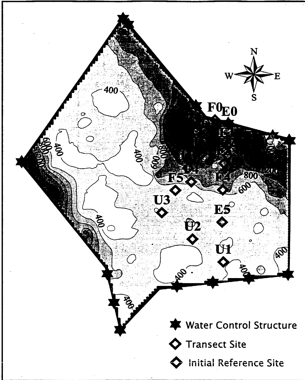
Figure 5-1. Locations of gradient transect monitoring sites established across phosphorus gradient in WCA-2A, as shown on a sediment contour map. Sediment contours provide P concentrations as mg/kg in the upper 10 cm of sediment, developed using a combination of District, DUWC and USEPA data
